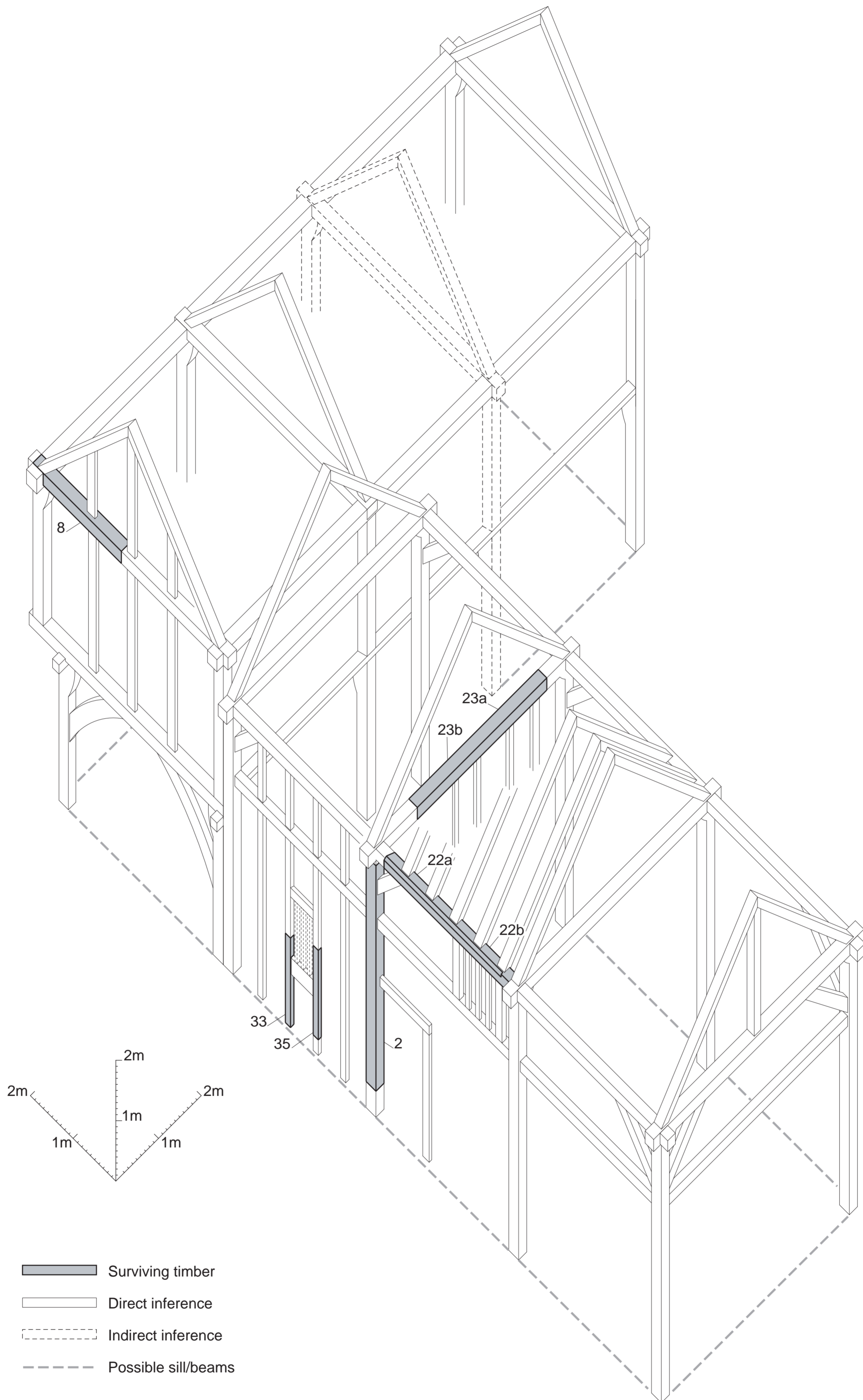
Manor Farm House, Thorpe on the Hill, Lincolnshire Axonometric projection view from South-East
