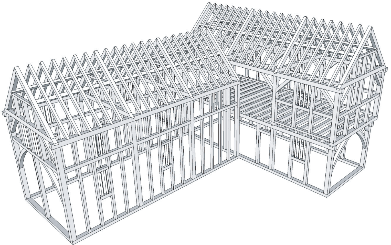
3D solid model drawn in Google Sketchup
